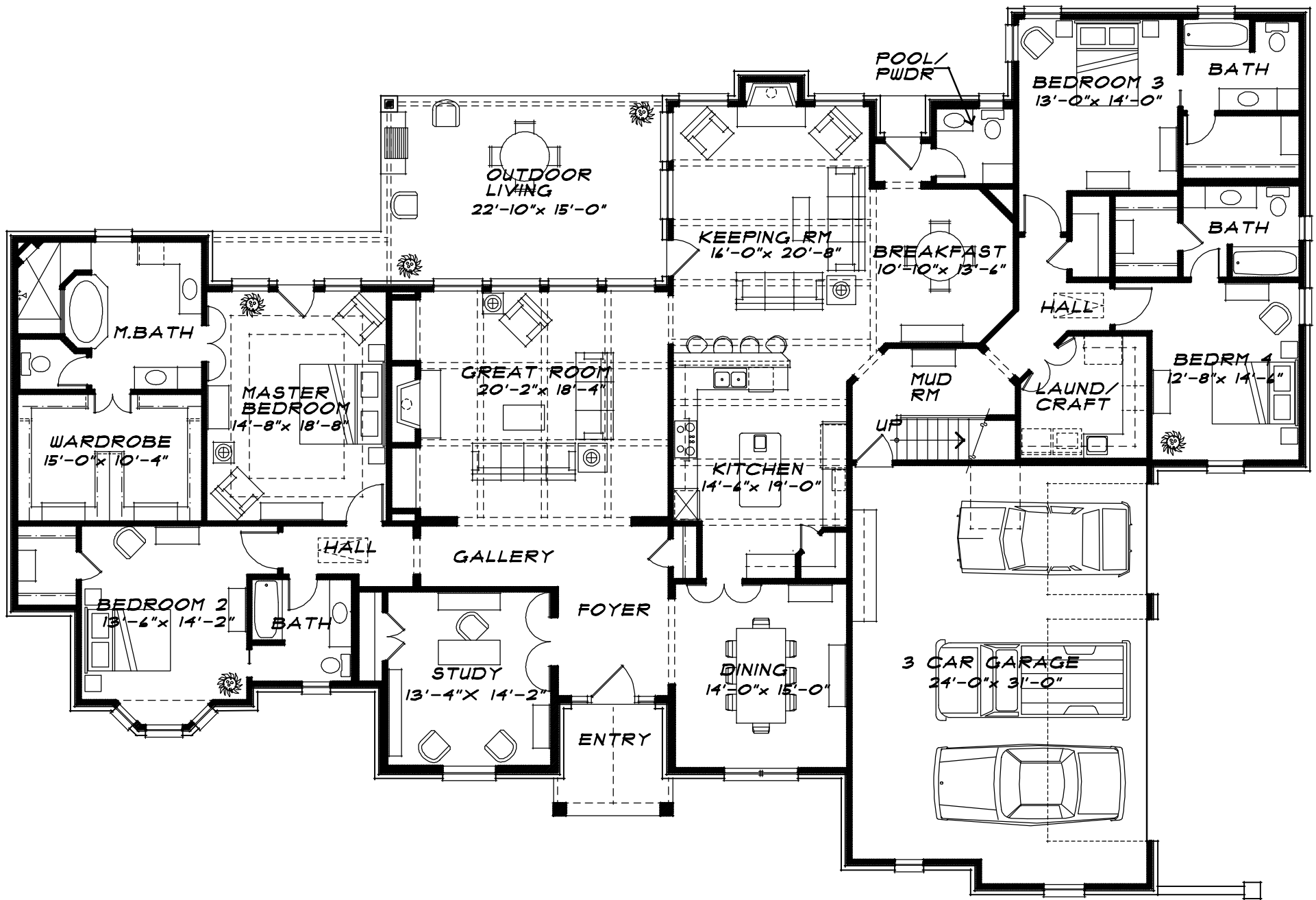
FLOOR PLAN TOTAL A/C AREA = 4013 SQ FT
